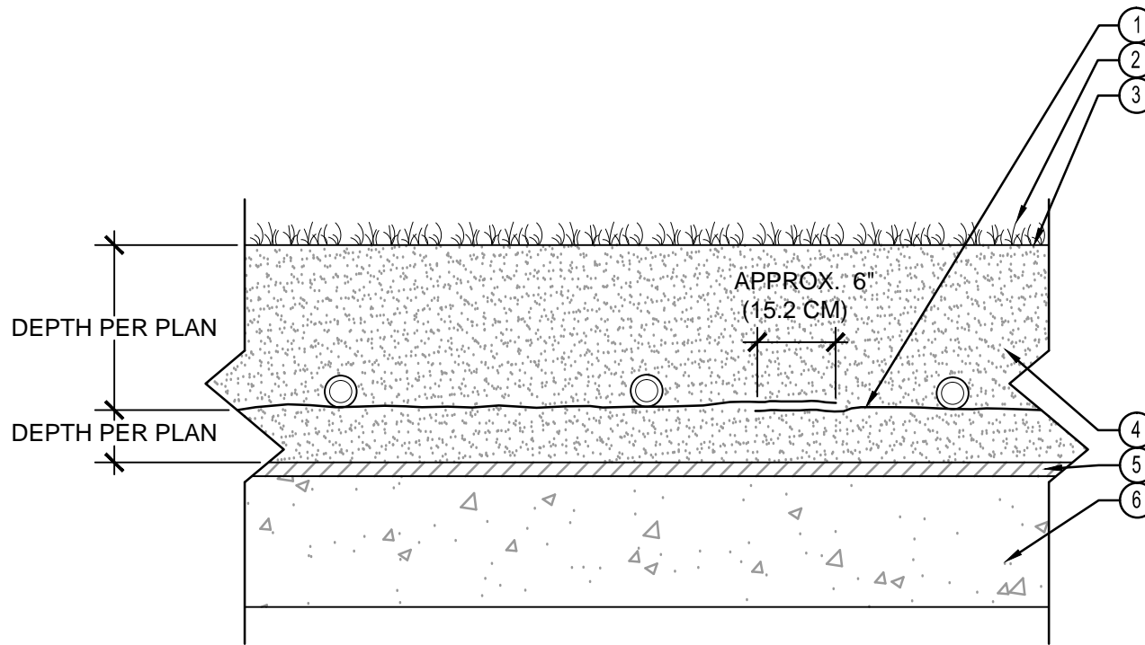
XX ECO-MAT - GREEN ROOF SECTION huter HM.EM.04
