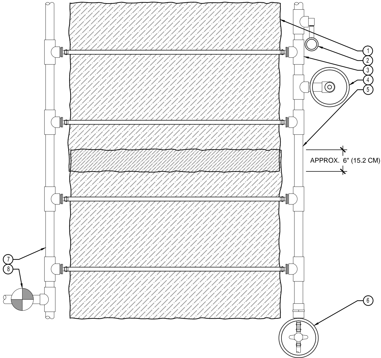
XX ECO-MAT - PLAN VIEW WITH PVC HEADER AND EXHAUST AT MAT GRADE Hunter HM.EM.02
