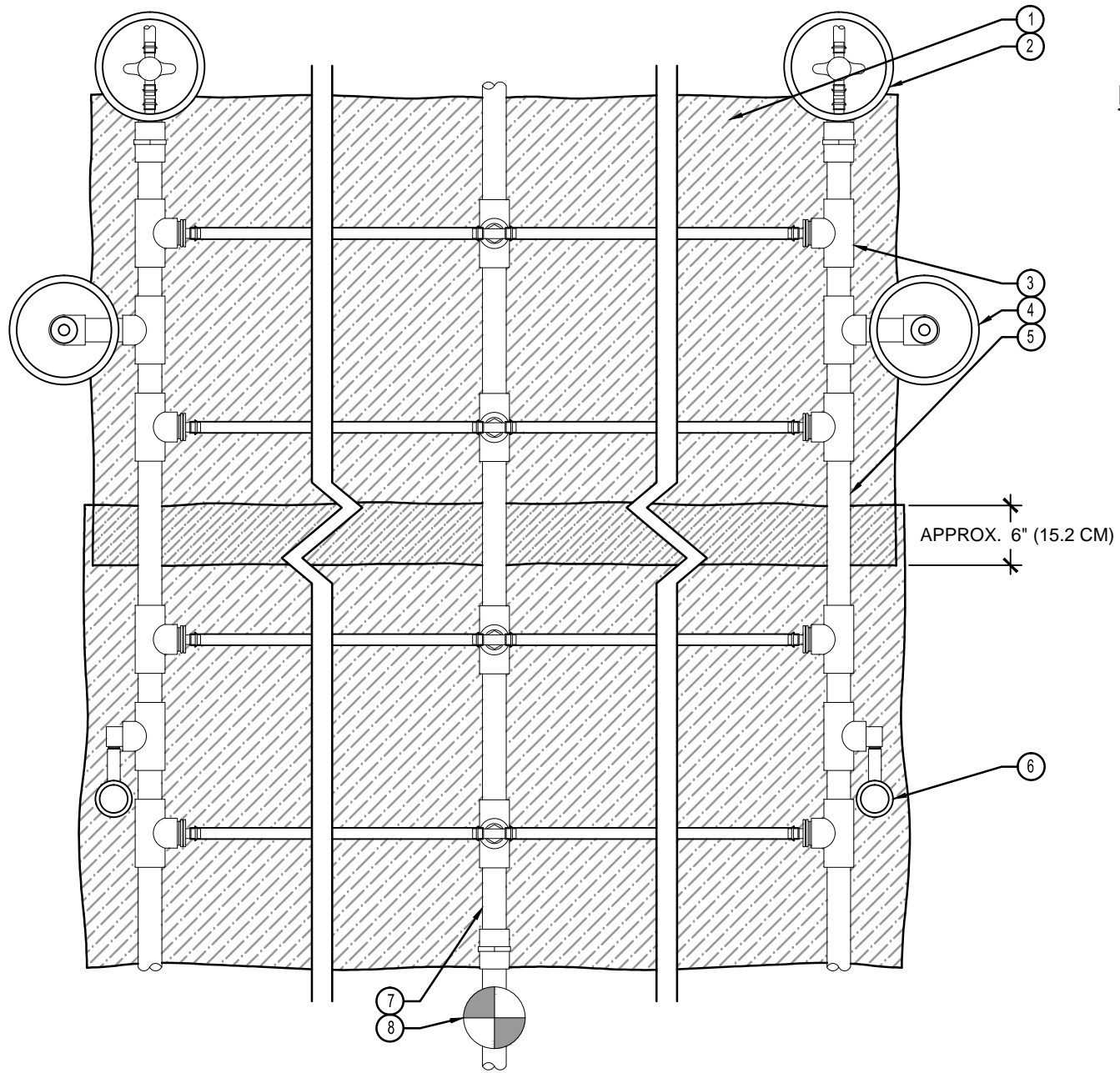
XX ECO-MAT - PLAN VIEW WITH PVC HEADER AND EXHAUST AT MAT GRADE CENTER FEED Hunter HM.EM.21
