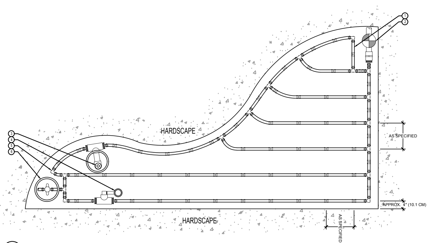
XX HUNTER DRIPLINE - IRREGULAR PLANTED AREA Hunter HM.HDL.02
