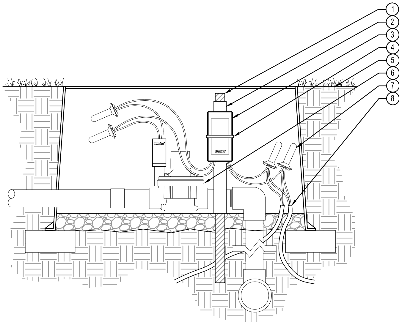
XX DUAL-1 DECODER ON STAKE Hunter C.DUAL.02
