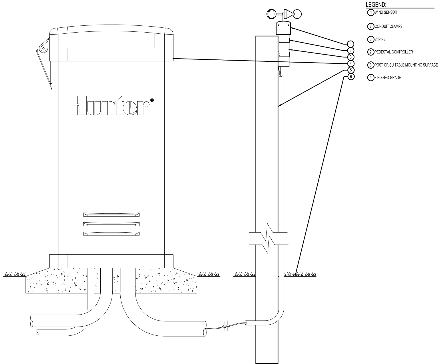
XX WIND-CLIK WITH GENERIC PEDESTAL CONTROLLER Hunter S.WC.02
